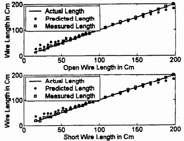
Fig. 7. Twin lead results with open and short.
